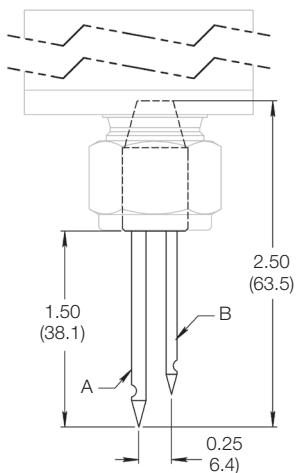
병렬형(Side-by-Side) 니들
