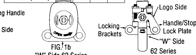
FIG. 1b "W" Side 62 Series Oval Handle Orientation
