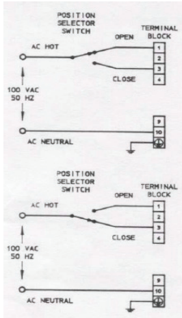
Control Signal Configuration
