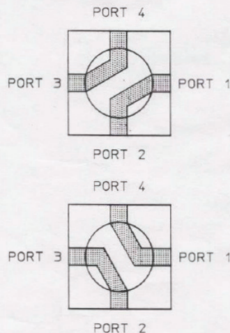
Resulting Valve Stem Position
