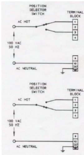
Control Signal Configuration
