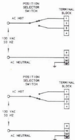
Control Signal Configuration
