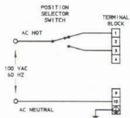
Control Signal Configuration
