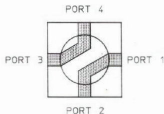
PORT 1 PORT 2
