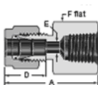
ISO/BSP Tapered Female Thread (RT)
