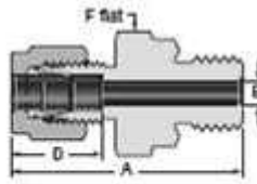
ISO/BSP Parallel Thread (RP)
