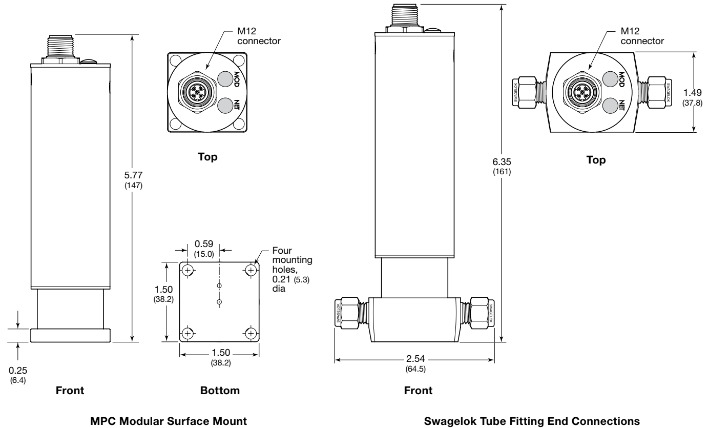
Fig. 4 Product Dimensions
