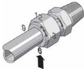
Mark the nut at 6 o'clock
