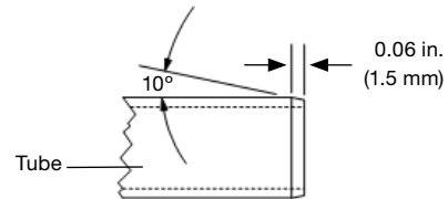
Chamfer tubing larger than 1 in. with a file
