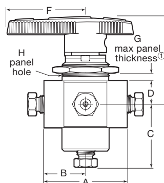
5-Way Valve
