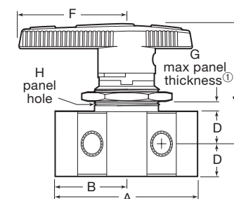
6-Way Valve
