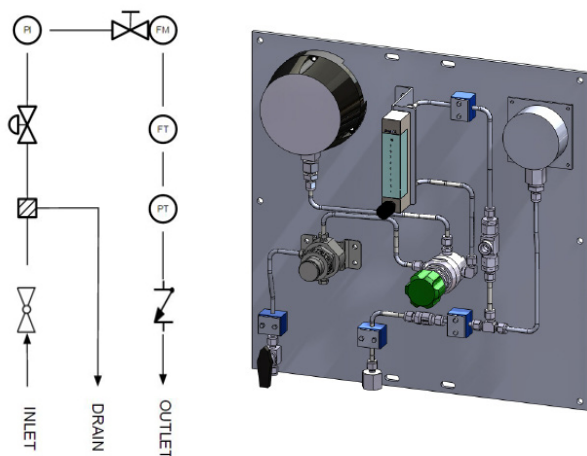
API 682 PLAN 74 - Single
