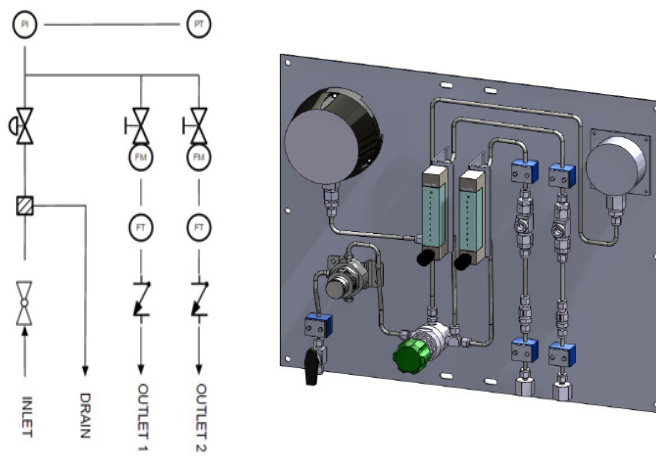
API 682 PLAN 74 - Dual
