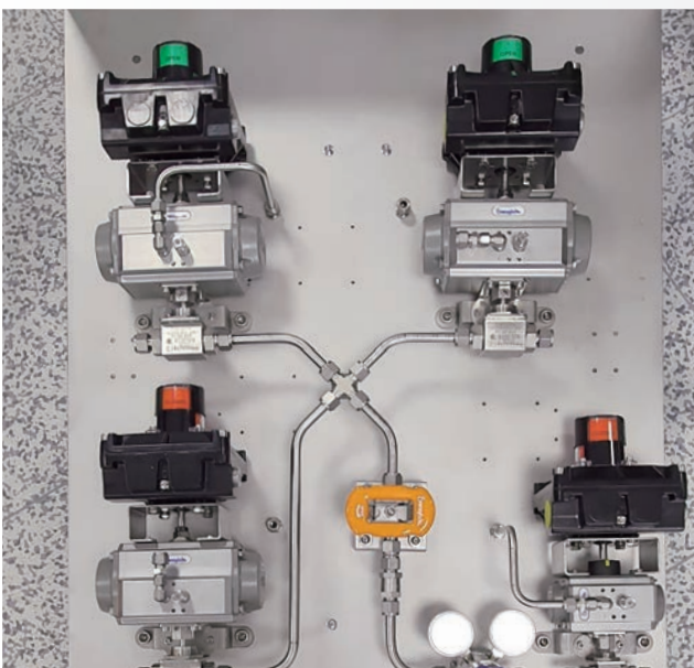
Control panel in kill system
