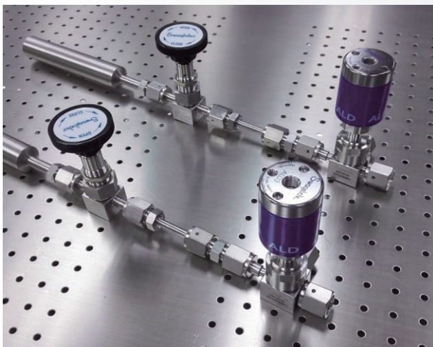
Gas & Liquid Sampling Panel
