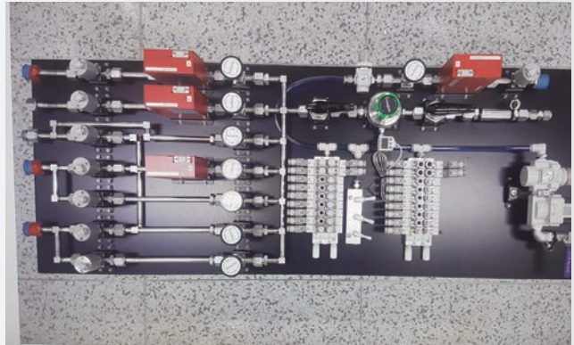
Sampling cylinder assembly
