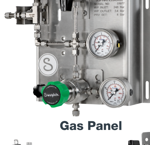
Gas Panel
