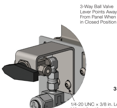
3-Way Ball Valve
