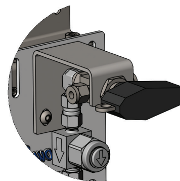
3-Way Ball Valve (lockable)
