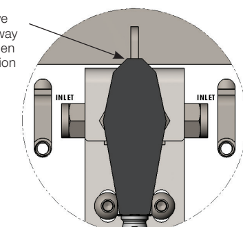
3-Way Ball Valve in Closed Position
