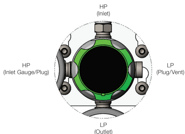
KPR E-Pattern Port Orientation (Top-to-Bottom Flow)
