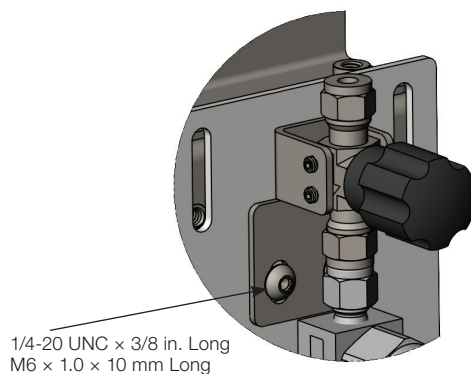
Multiturn Needle Valve
