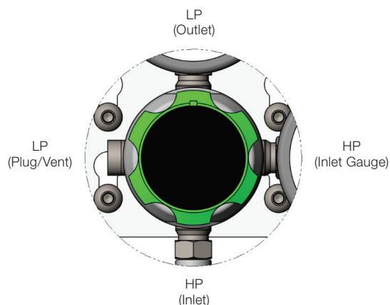
KPR E-Pattern Port Orientation (Bottom-to-Top Flow)
