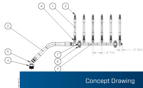
CAD model
