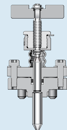
Bolted OS&Y Bonnet
