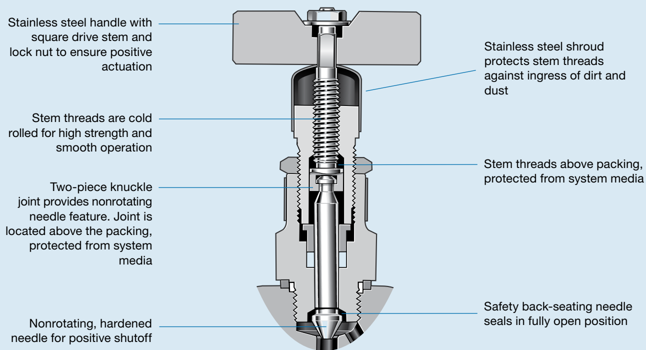
Screwed Bonnet
