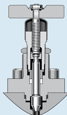
Bolted Bonnet
