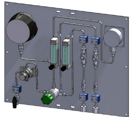
API 682 Plan 74 - Dual
